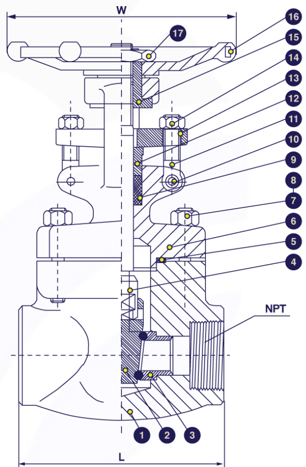
Threaded End SS316 Gate Valves 800 PSI
